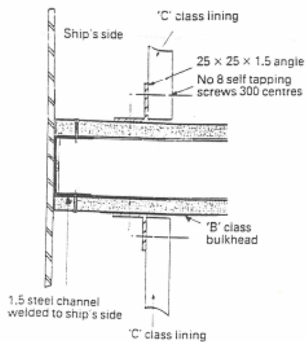
Connection between 'B' class bulkhead and 'C' class lining
