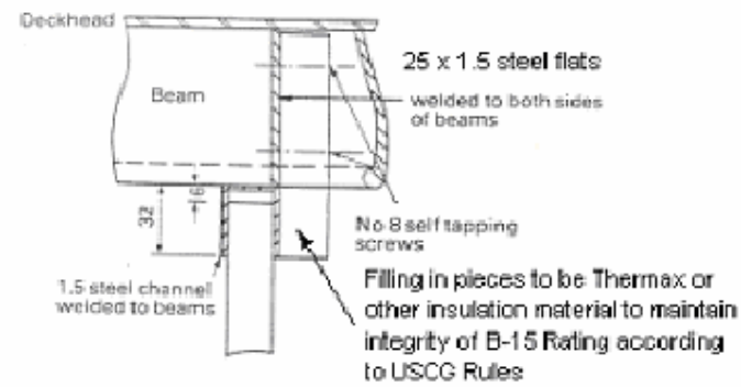
Bulkhead connection to deckhead showing filling in pieces between beams
